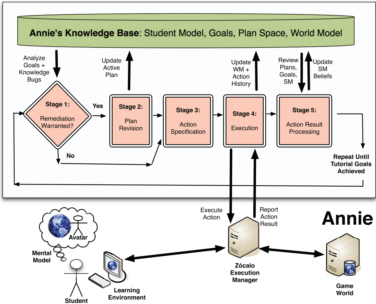
Fig. 6. Execution data flows.
