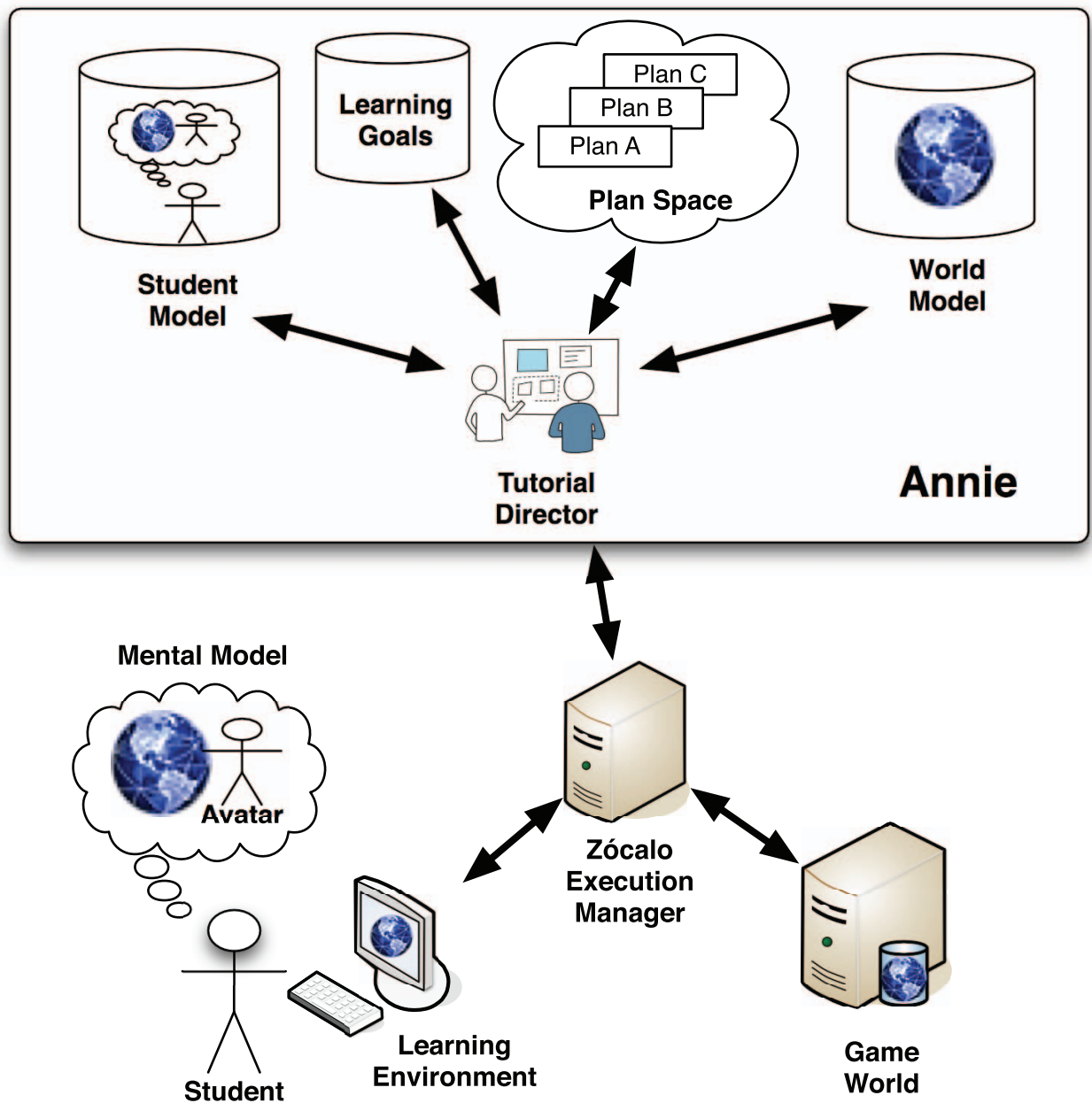
Fig. 4. System architecture.
