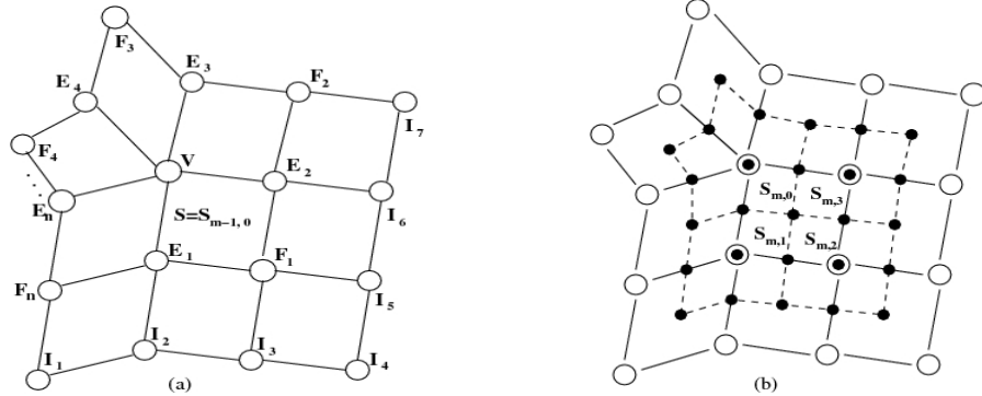
Figure 1: (a) Control vertices that influence an extra-ordinary patch. (b) New control vertices (solid dots) generated after a Catmull-Clark subdivision.
