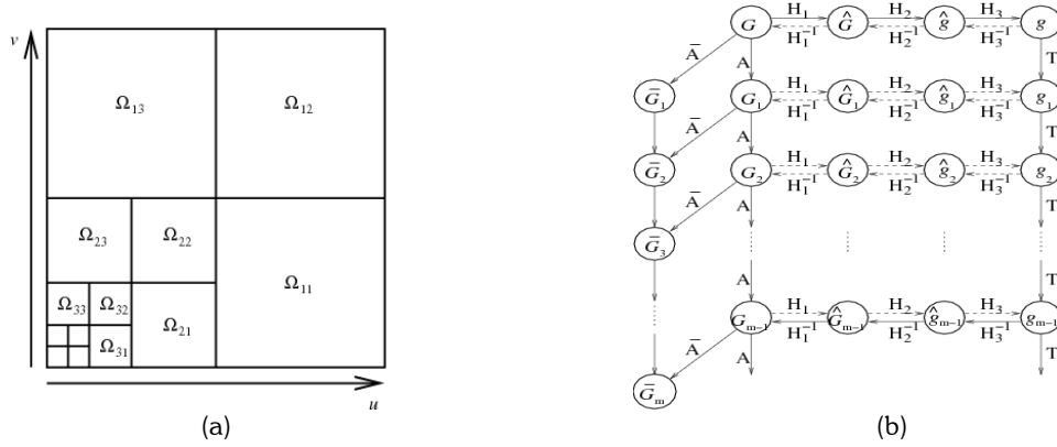
Figure 2: (a) \Omega -partition of the unit square [14]; (b) The extended subdivision diagram.
