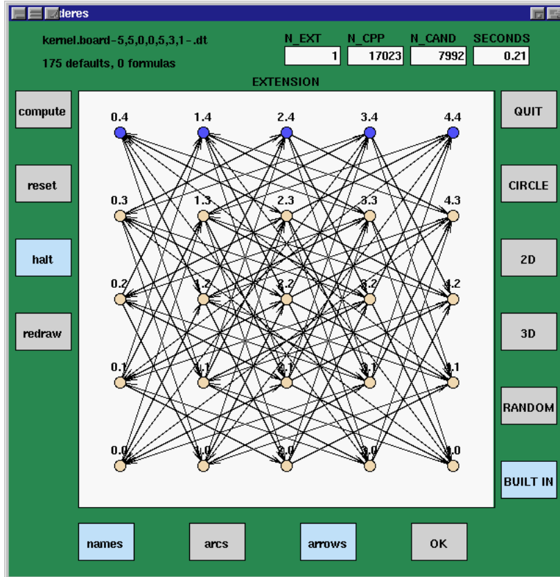
Figure 7: A kernel in graph board(5, 5, 0, 0, 5, 3, 1) .
