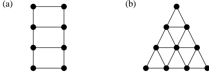
Figure 9: (a) Ladder graph; (b) Simplex graph
