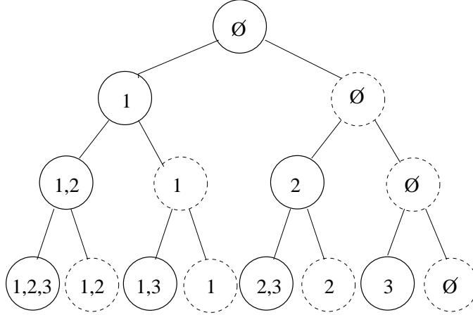
Figure 2: Generating all subsets of X = \{1, 2, 3\} .
