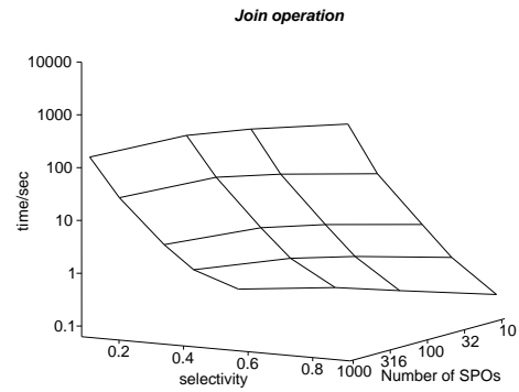
Figure 20. Effect of number of SPOs and selectivity on join operation.
